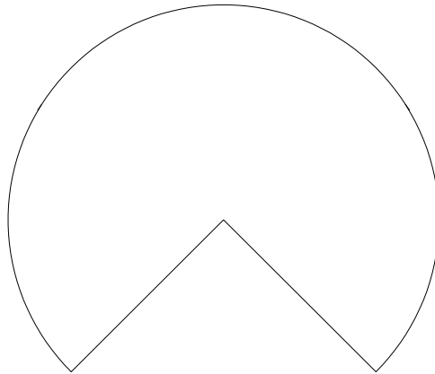
CORNER ROUND 925019 2 3/16" X 2 1/2"
