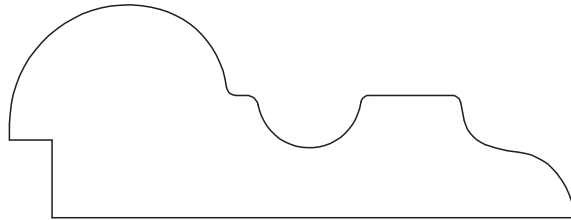
BASE CAP 22503 15/16" X 2 1/2"
