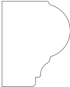
NOSING 9157 1 9/16" X 1 1/4"
